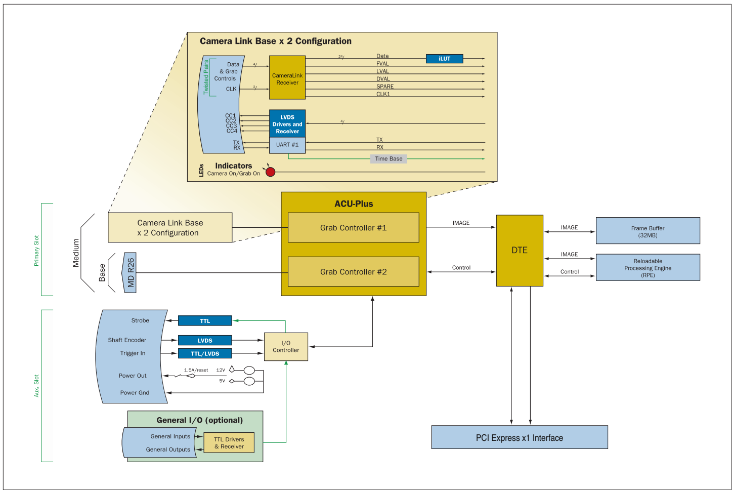
X64-CL Express – Functional Block Diagram
