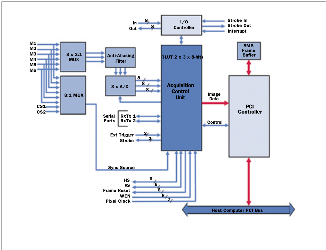
PC2-Vision Functional Block Diagram
